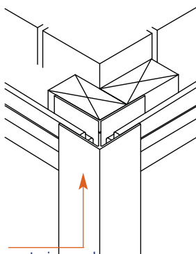
Profile of an exterior angle 2 part Int/Ext corner trim (5513)
