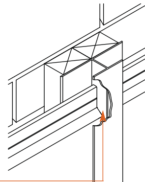
Profile of a 2 part Centre Joint Trim (5509)
