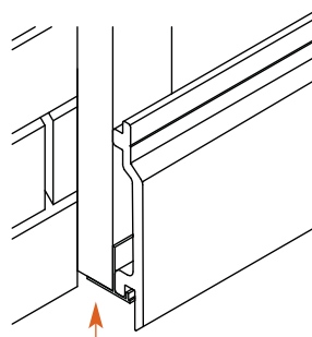
Profile of Starter Trim with batten cover (5504)
